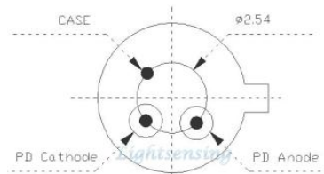
Type B PIN description Bottom View
